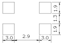
7060 PAD LAYOUT
