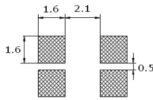
4520 PAD LAYOUT
