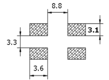
1513 PAD LAYOUT
