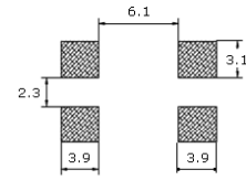
1211 PAD LAYOUT
