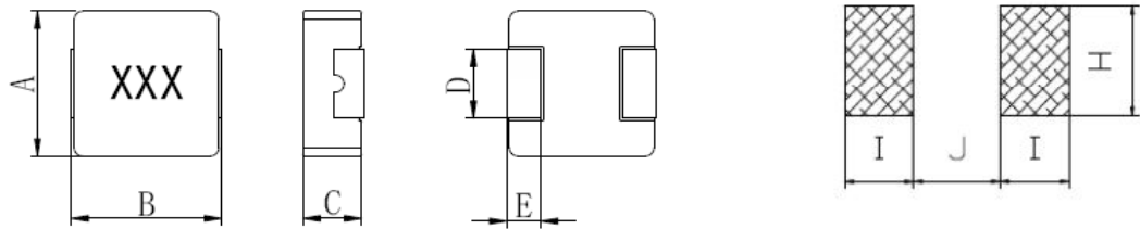
LAND PATTERN
