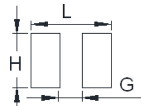
LAND PATTERN
